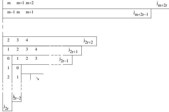
FIGURE 5. Construction of \lambda(c) = \mathcal{J}_m(\xi(c), \eta(c))
